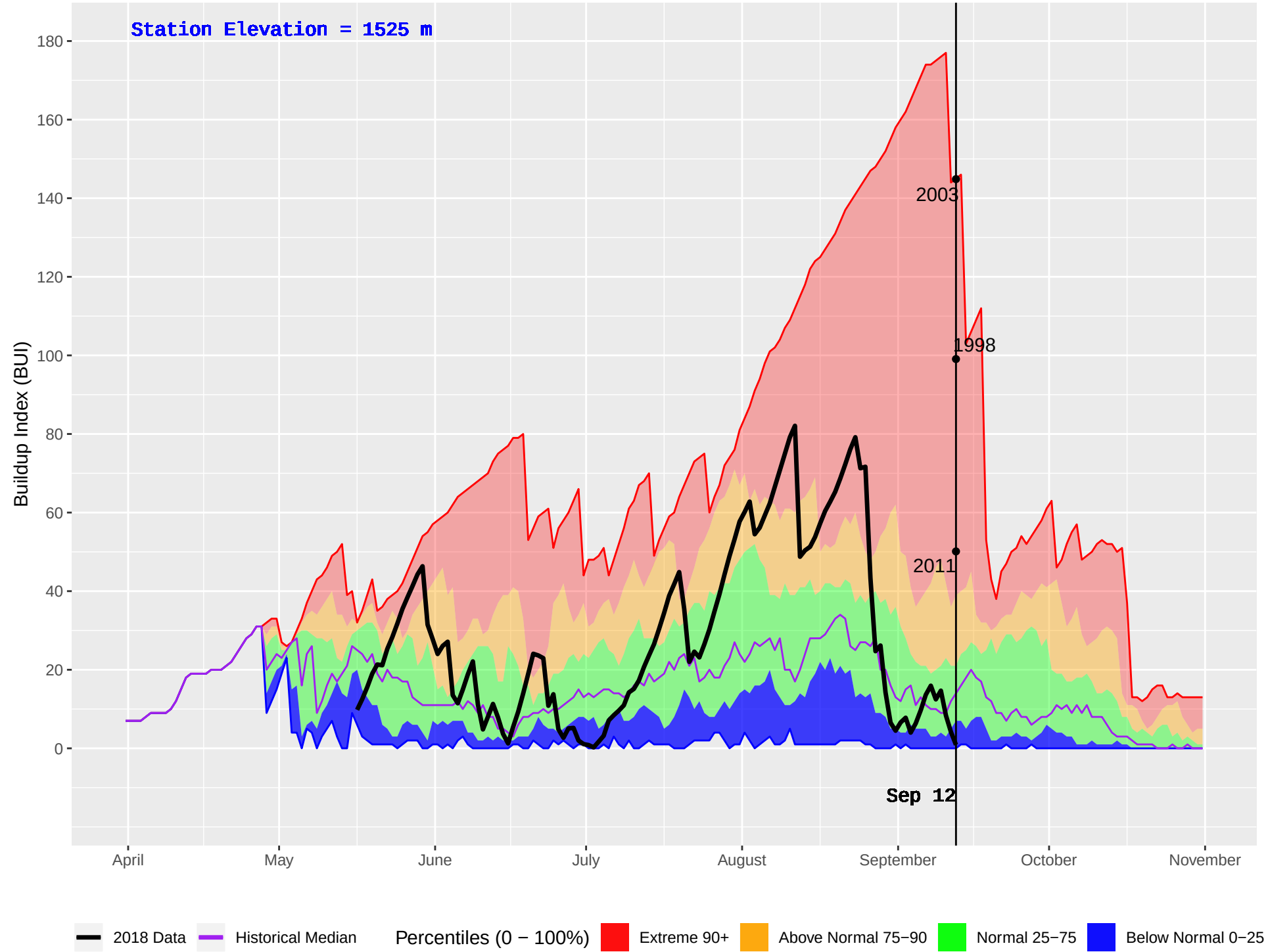
HARBOUR LAKE (250) : Historical (1989–2016) and Current (2018) Daily Buildup Index (BUI)
