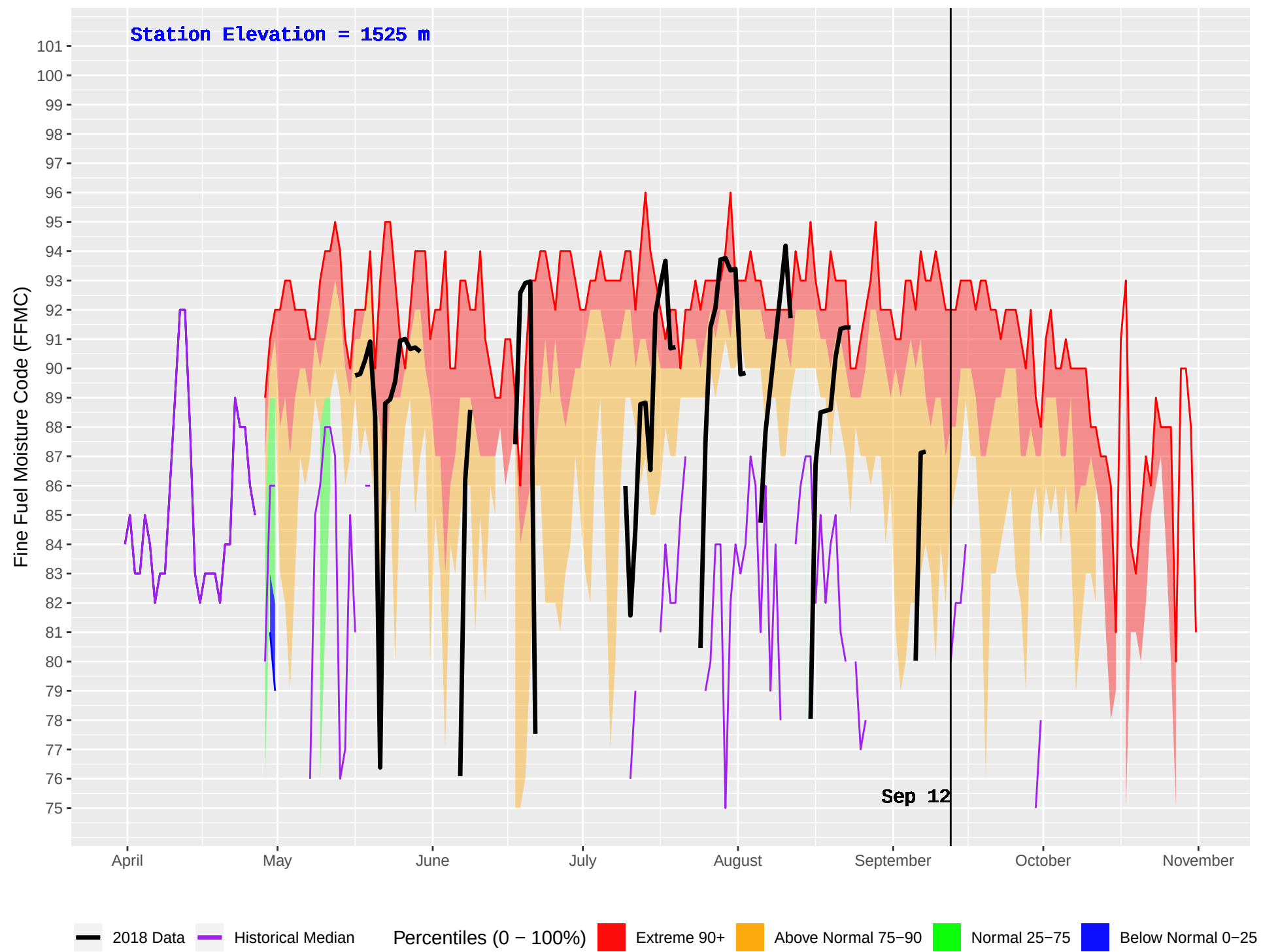
HARBOUR LAKE (250) : Historical (1989–2016) and Current (2018) Daily Fine Fuel Moisture Code (FFMC)
