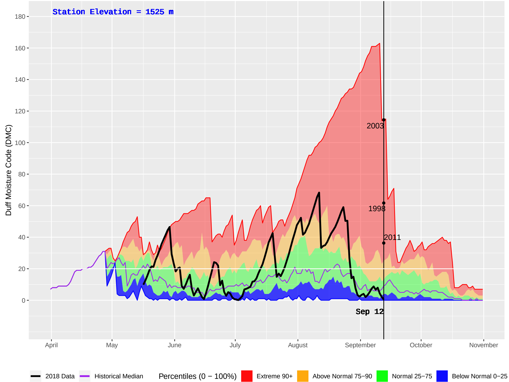
HARBOUR LAKE (250) : Historical (1989–2016) and Current (2018) Daily Duff Moisture Code (DMC)
