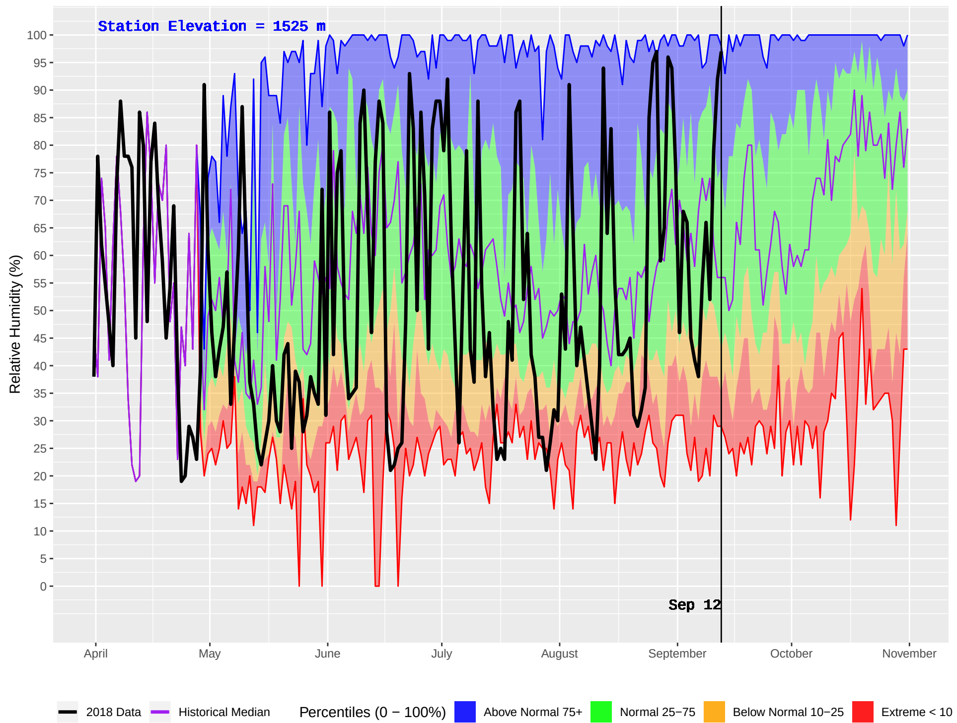
HARBOUR LAKE (250) : Historical (1989–2016) and Current (2018) Daily Relative Humidity
