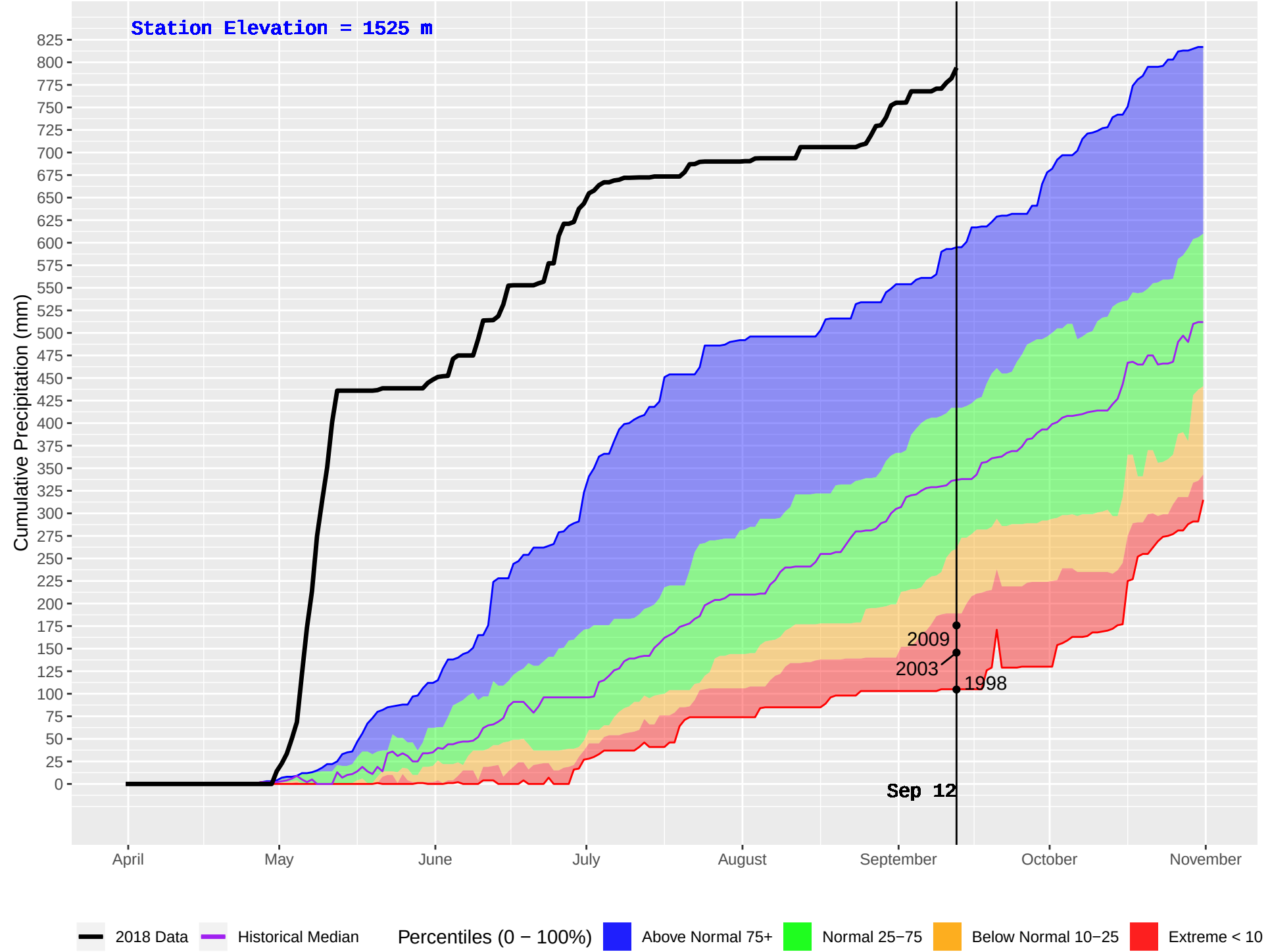
HARBOUR LAKE (250) : Historical (1989–2016) and Current (2018) Daily Cumulative Precipitation
